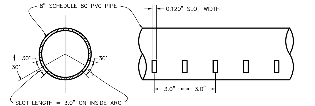
DETAIL 'A' LEACHATE PIPE SLOTS NOT TO SCALE
